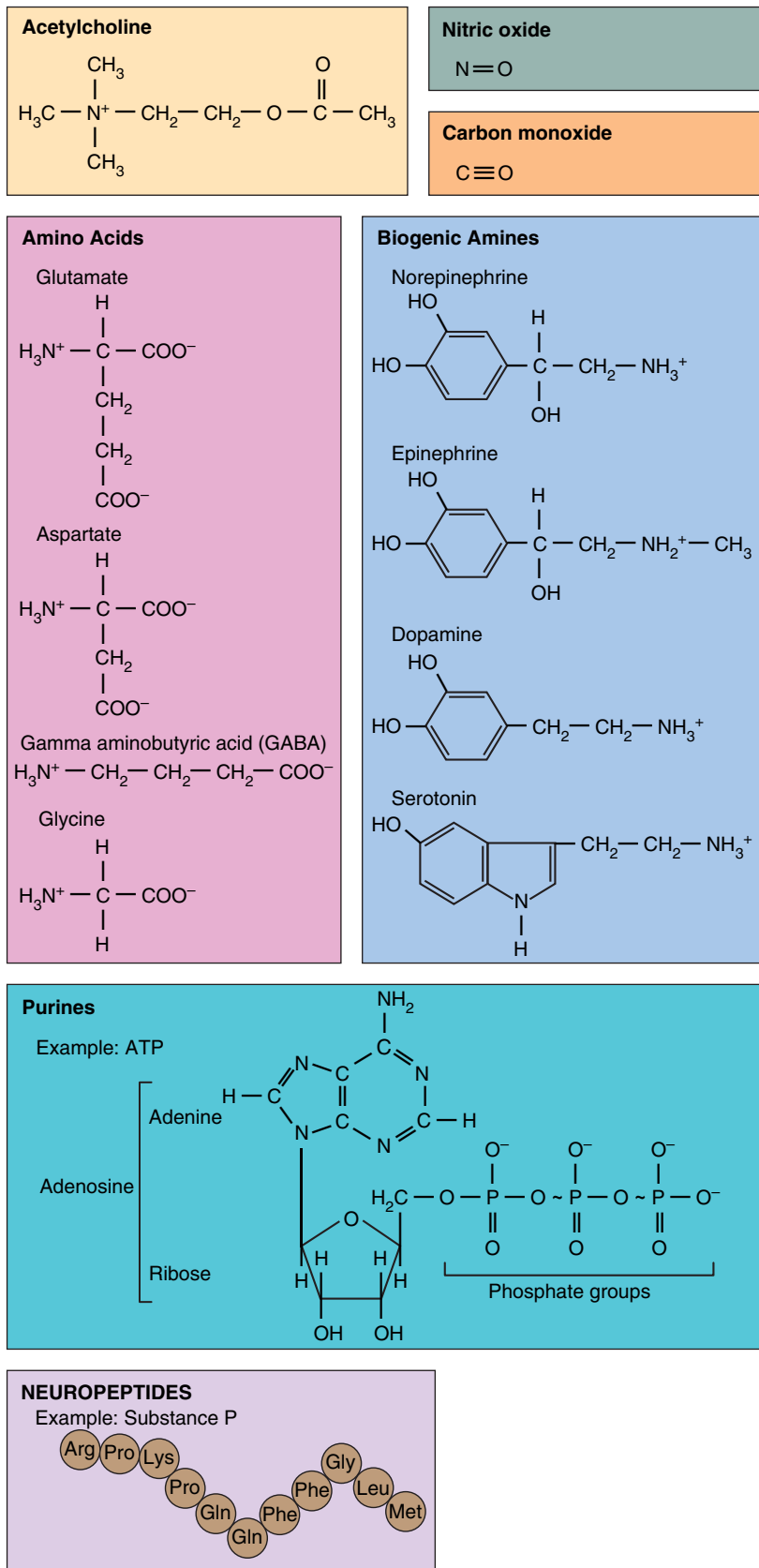
FIGURE 12.27 Neurotransmitters. Neurotransmitters are divided into two major classes based on size: small-molecule neurotransmitters and neuropeptides. The neuropeptide shown is substance P, which consists of 11 amino acids linked by peptide bonds in the following order: arginine (Arg), proline (Pro), lysine (Lys), proline, glutamine (Gln), glutamine, phenylalanine (Phe), phenylalanine, glycine (Gly), leucine (Leu), and methionine (Met).
