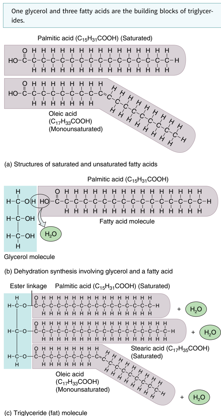
FIGURE 2.17 Fatty acid structure and triglyceride synthesis. Each time a glycerol and a fatty acid are joined in dehydration synthesis (b), a molecule of water is removed. Shown in (c) is a triglyceride molecule that contains two saturated fatty acids and a monounsaturated fatty acid. The kink (bend) in the oleic acid occurs at the double bond.
